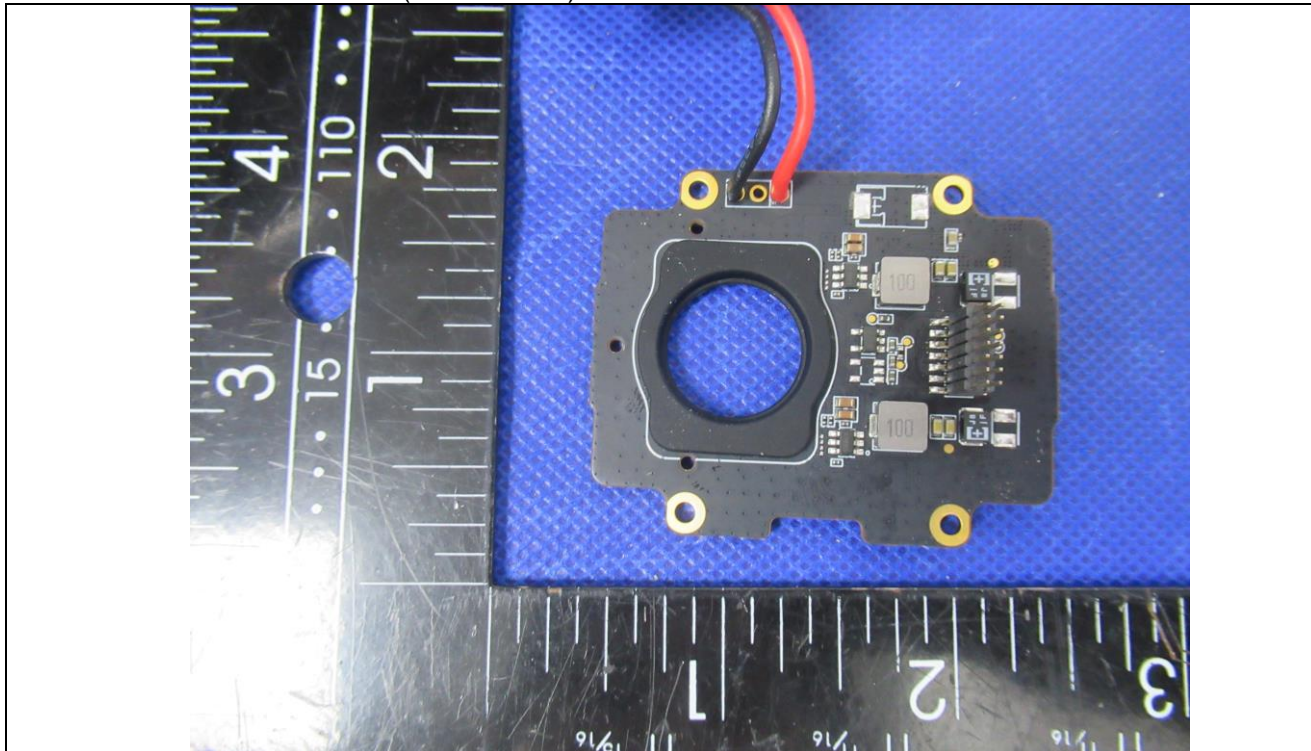
Details of: DCAM560C Lite (Internal view)
