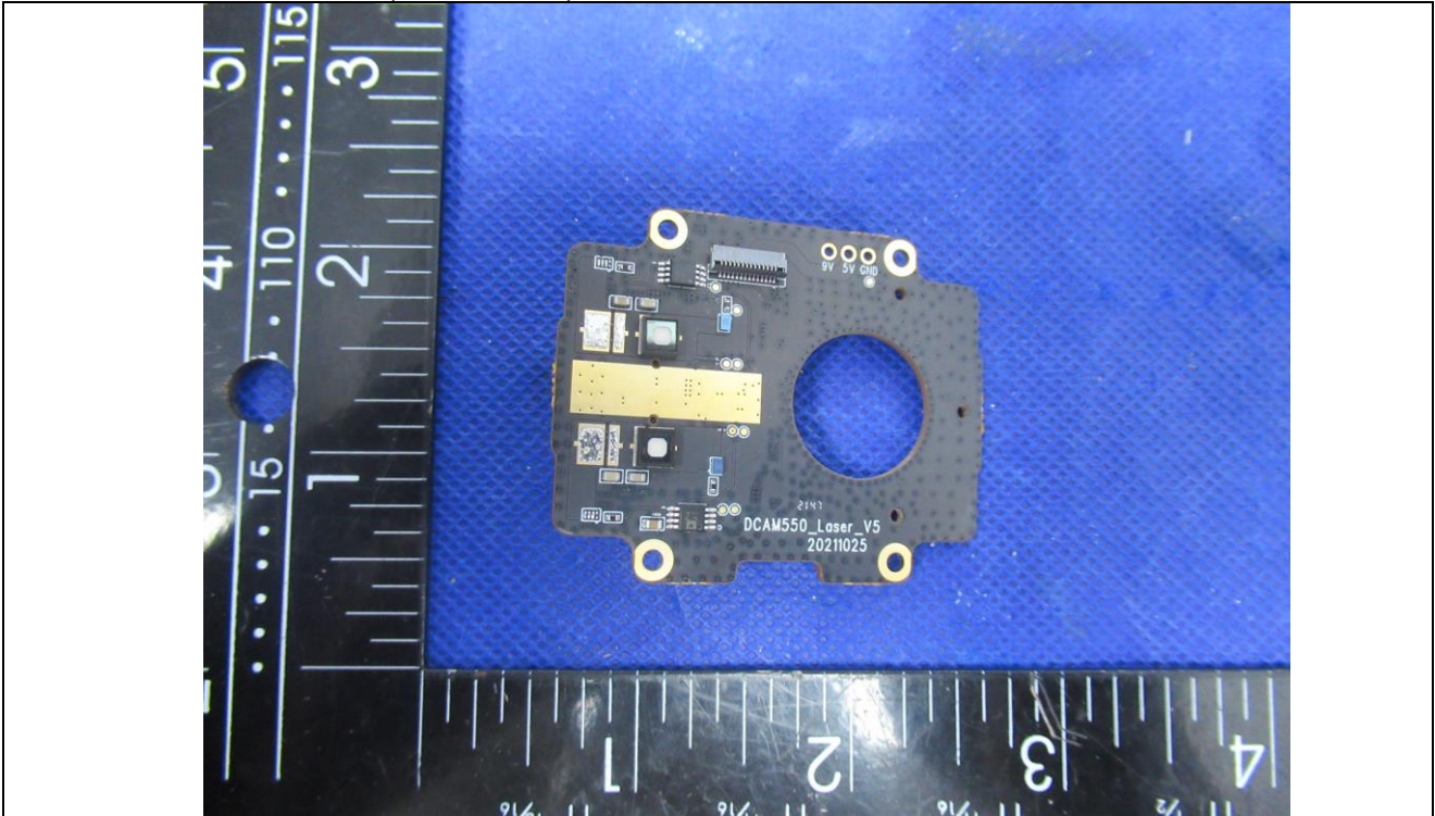
Details of: DCAM550-P (General view)
