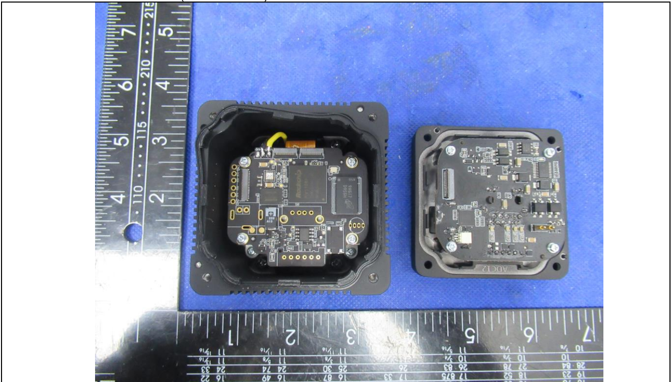
Details of: DCAM550-P (Internal view)
