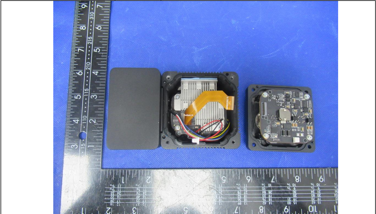
Details of: DCAM560C Pro (Internal view)
