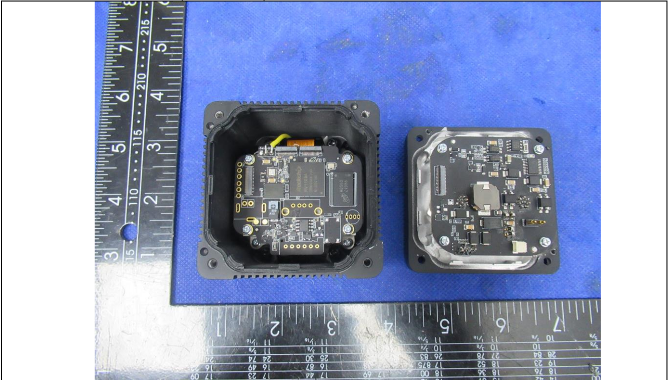
Details of: DCAM560C Lite (General view)
