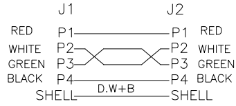
Wiring Diagram
