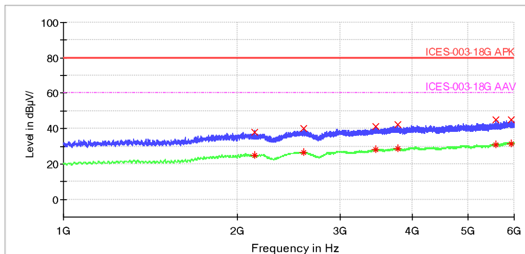
ICES RE-1-6GHz-A-3115-Pre
